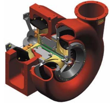
TSI Turbocharger
